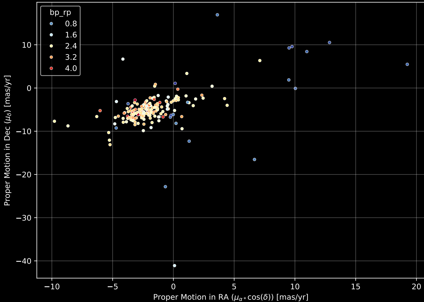
APOGEE DR17 Field: [053+04] Proper Motion Diagram (n= 189)
