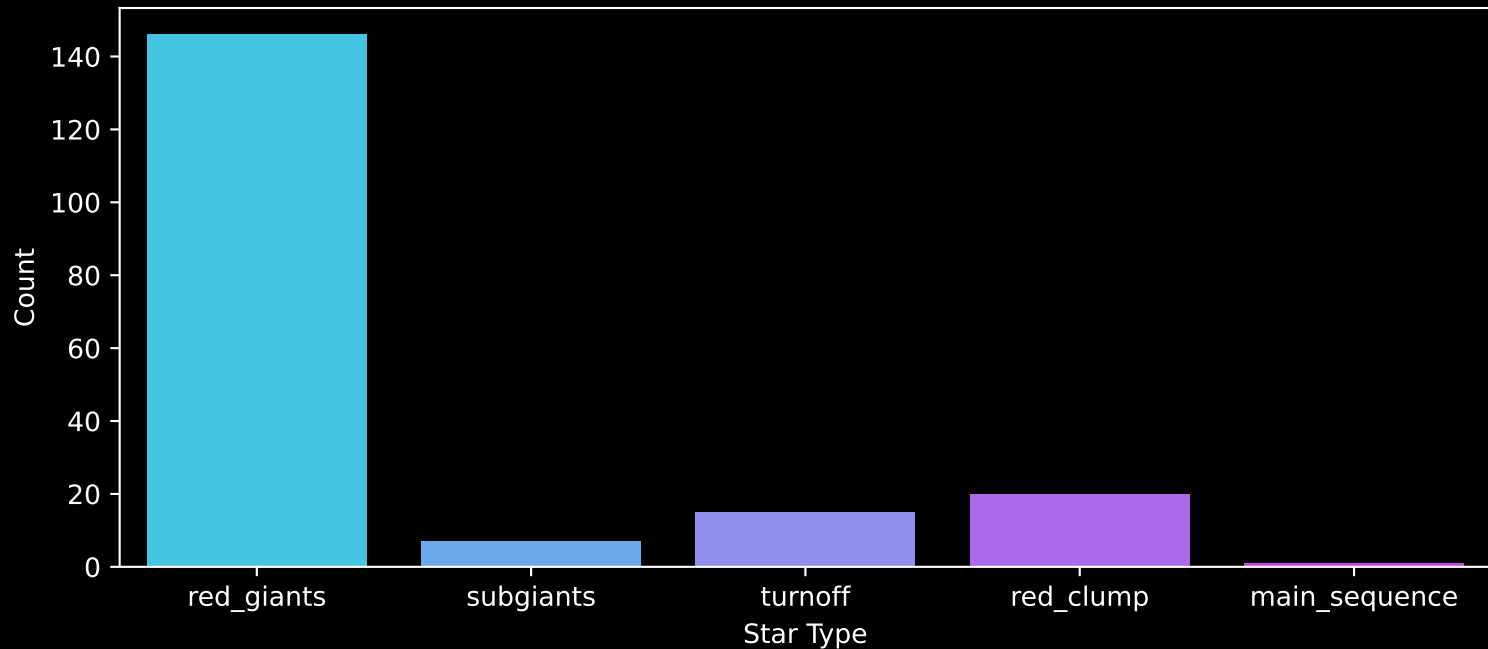
APOGEE DR17 Field: [053+04] Count plot of Star Type
