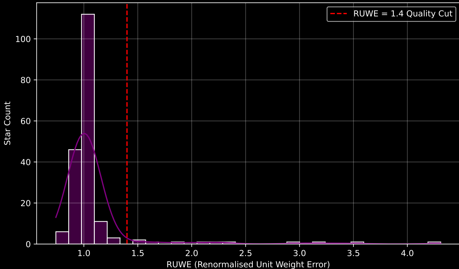
GAPOGEE DR17 Field [053+04] RUWE Distribution (n= 189)
