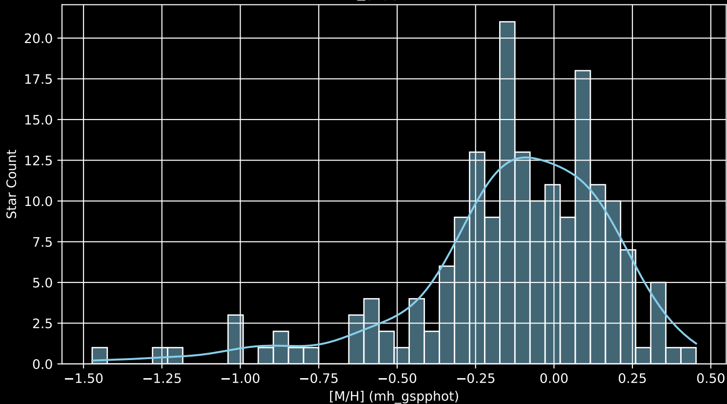
APOGEE DR17 Field: [053+04 [M/H] (mh_gspphot) (n= 182)
