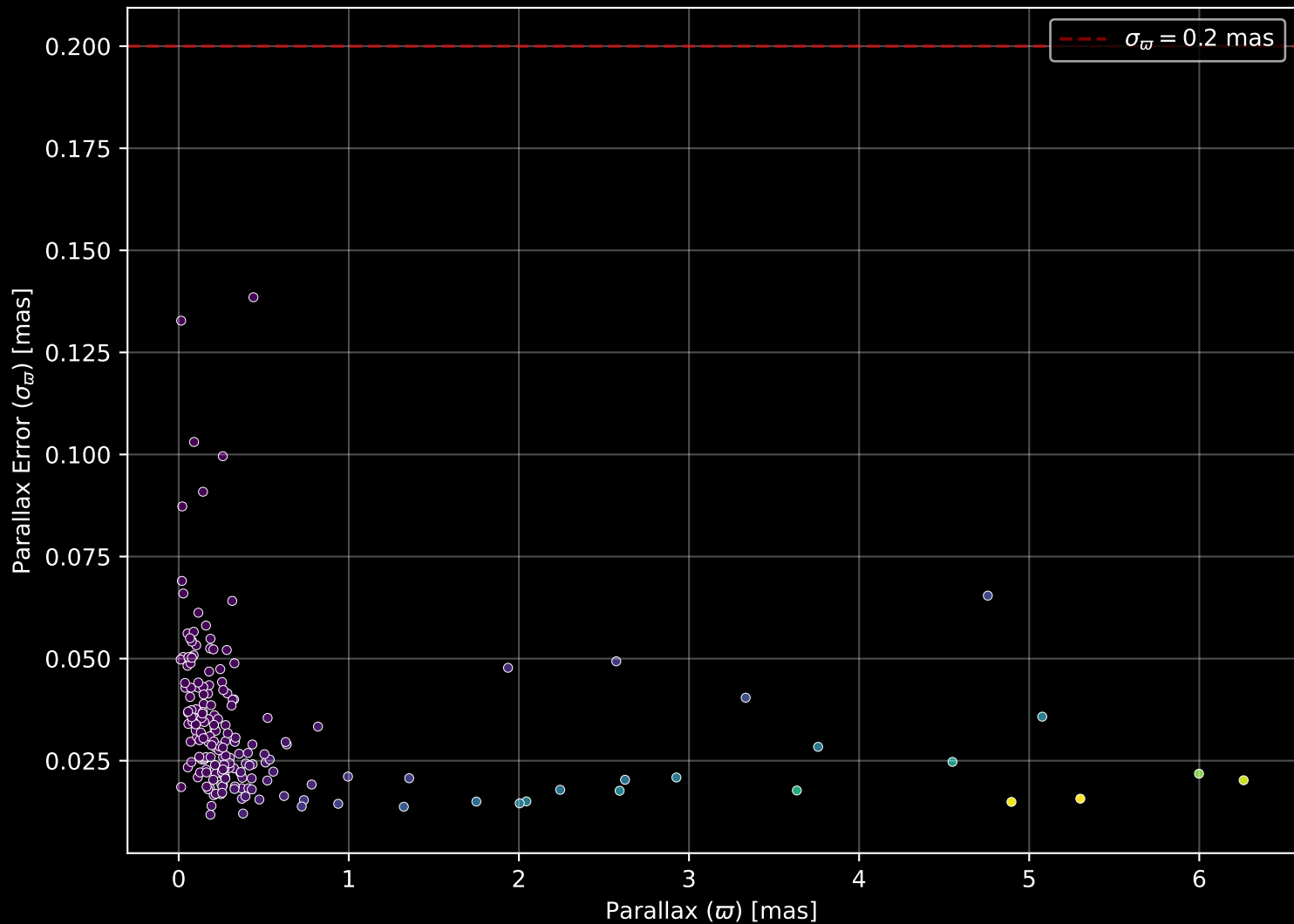
APOGEE DR17 Field: [053+04] Parallax Quality (n= 189)
