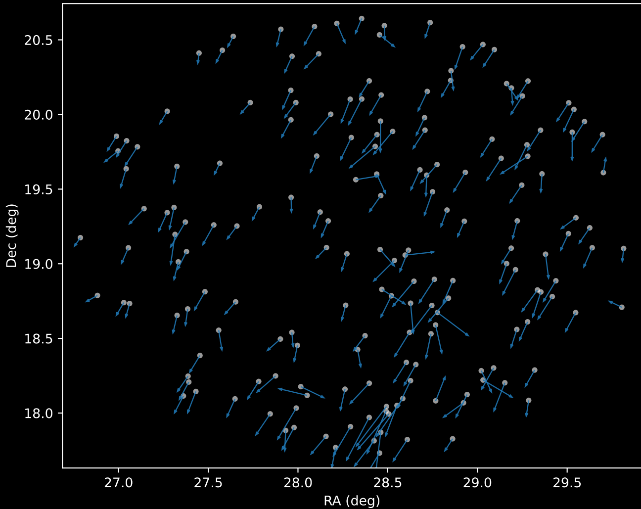
APOGEE DR17 Cluster 0 Proper Motion Vectors (n=177)
